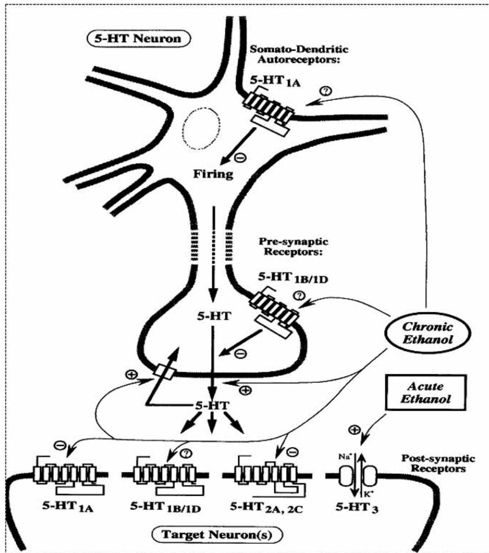
Fig. (1). Effect of chronic and acute effect of ethanol on the various 5-HT receptor subtypes, (+) positive effect and (-) negative effect. (Nevo and Hamon, 1995).
