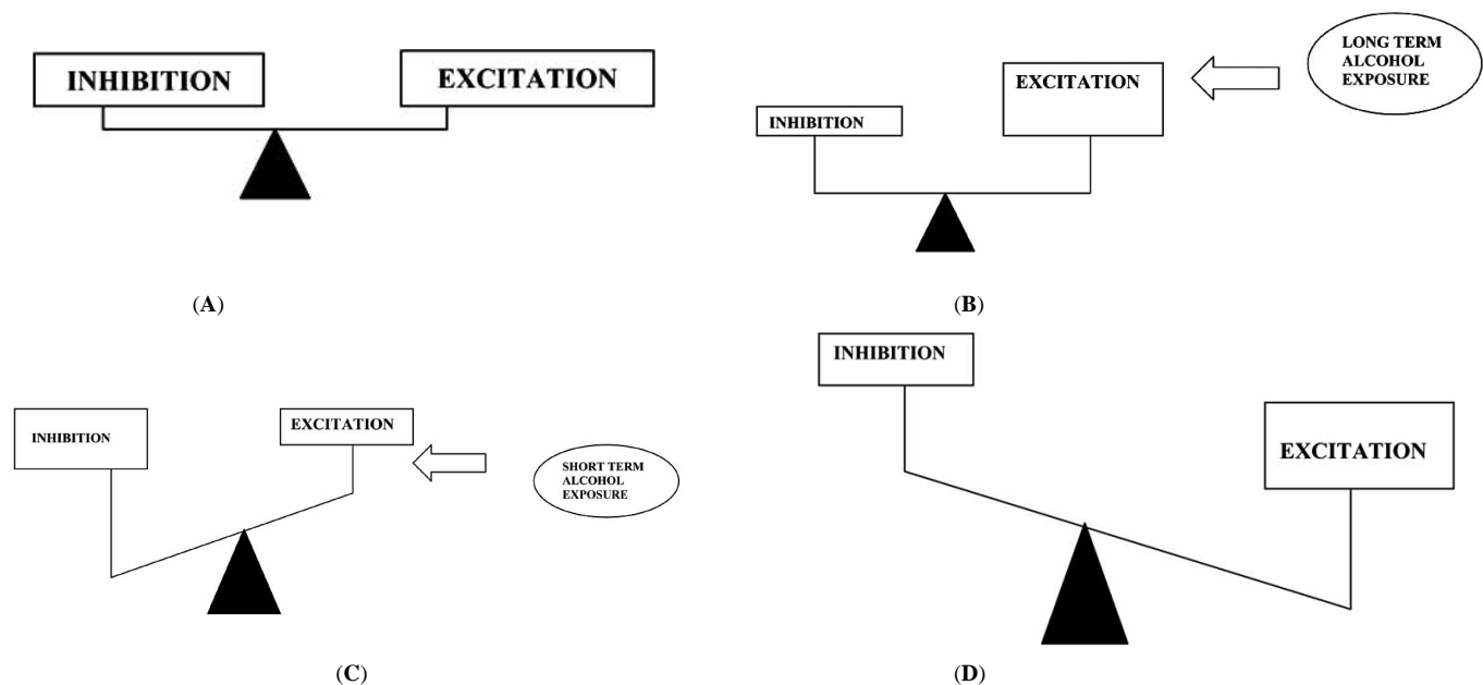
Fig. (2). (A). Under normal conditions, a balance exists between excitatory and inhibitory neurotransmission in the brain. (B). In long-term alcohol exposure, the brain attempts to restore equilibrium by compensating for the depressant effects of alcohol; thus, the brain decreases inhibitory neurotransmission and enhances excitatory neurotransmission. (C). Short-term alcohol exposure tilts the balance toward inhibition by both enhancing the function of inhibitory neurotransmitters and neuromodulators (i.e., GABA, glycine, and adenosine) and decreasing the function of excitatory neurotransmitters (i.e., glutamate and aspartate). (D). During alcohol withdrawal, the compensatory changes are no longer opposed by the presence of alcohol and the balance shifts toward a state of excessive excitation. This state of hyperexcitation is characterized by seizures, delirium, and anxiety in alcoholism. (Valenzuela, 1997).
