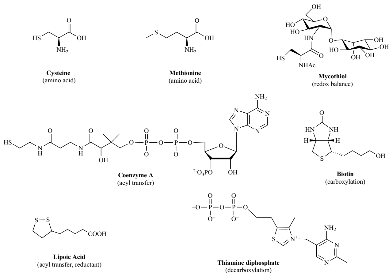
Fig. (1). Reduced sulfur-containing metabolites in mycobacteria.
