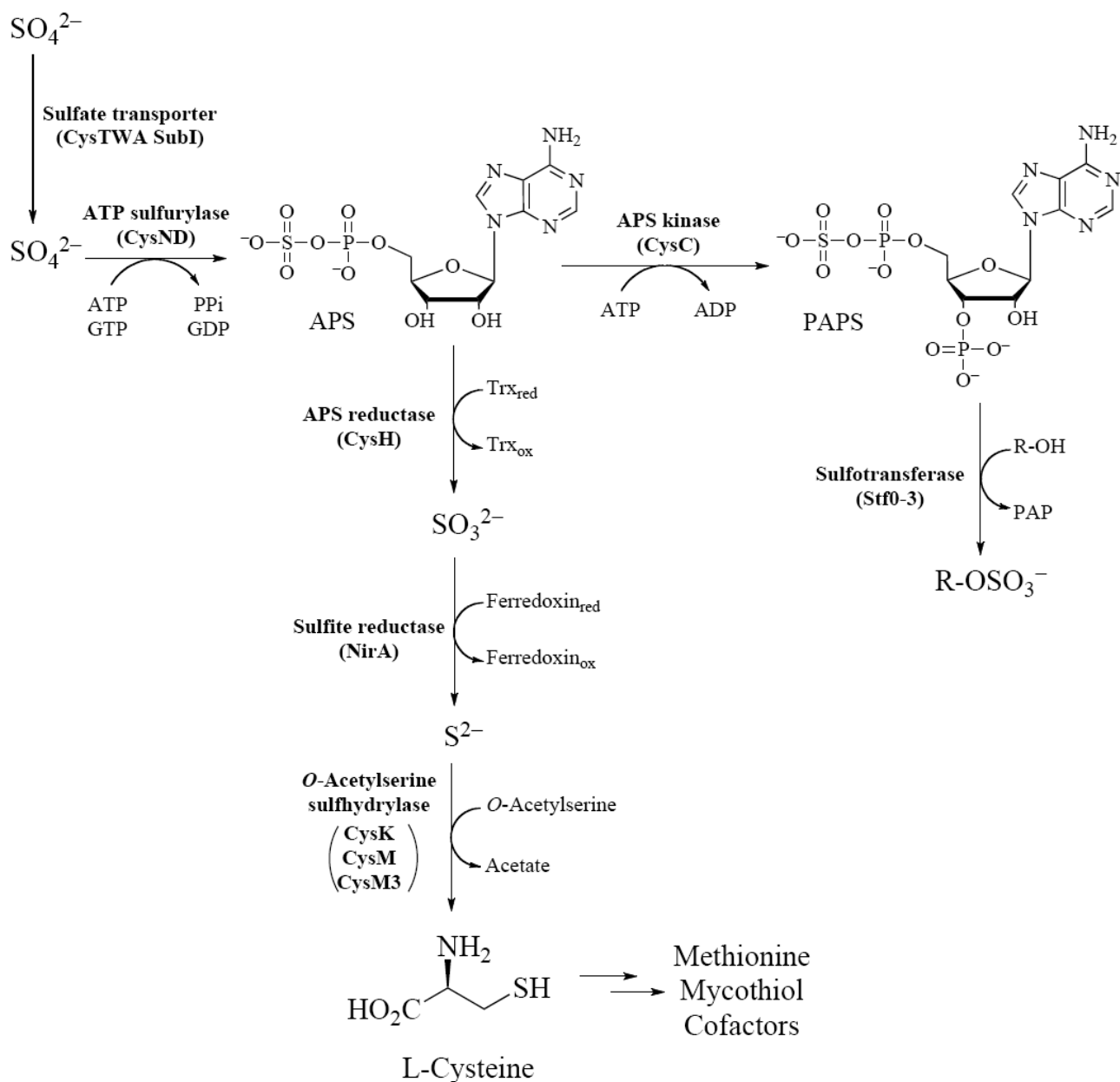
Fig. (3). The sulfate assimilation pathway in mycobacteria.
