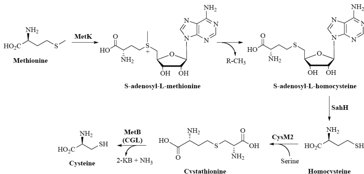
Fig. (7). Reverse transsulfuration pathway in mycobacteria.
