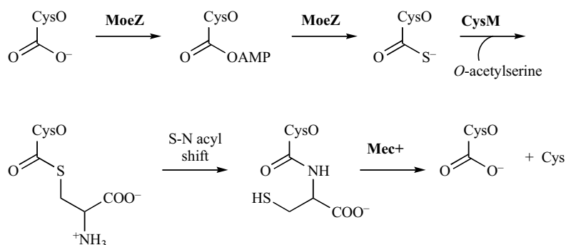
Fig. (4). Postulated alternate cysteine biosynthetic pathway [153].
