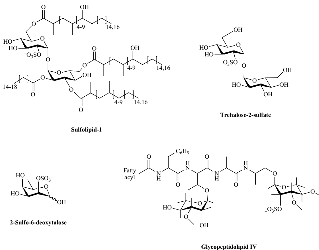
Fig. (2). Sulfated metabolites in mycobacteria.
