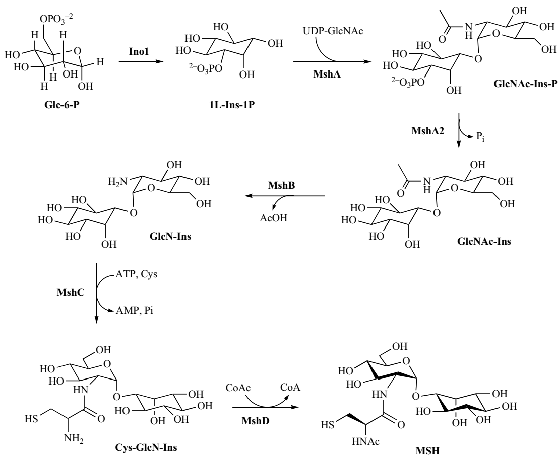
Fig. (5). MSH biosynthetic pathway.
