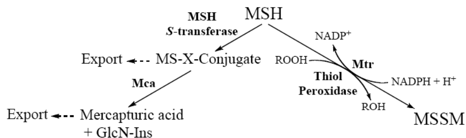
Fig. (6). MSH-mediated detoxification pathways.
